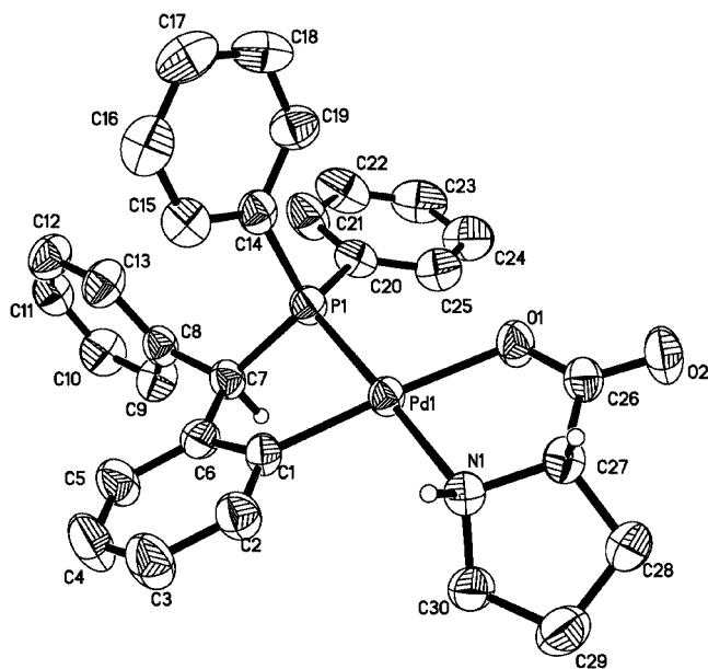
Figure 2. X-ray molecular structure of Z -( R C , S C , S N )- 4 .
