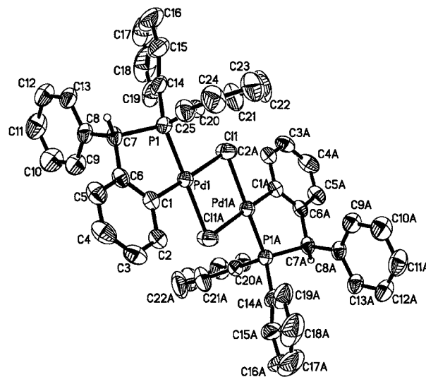
Figure 1. X-ray molecular structure of meso - 3 . Selected bond lengths [Å] and bond angles [°]: Pd1–C1, 2.017(3); Pd1–P1, 2.183(1); Pd1–Cl1, 2.441(1); Pd1–Cl1A, 2.407(1); C1–Pd1–P1, 79.43(8); C1–Pd1–Cl1, 174.43(8); C1–Pd1–Cl1A, 97.87(8); P1–Pd1–Cl1, 96.95(3); Cl1–Pd1–Cl1A, 97.87(8); Pd1–Cl1–Pd1A, 94.39(3).
