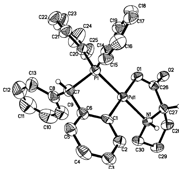
Figure 3. -ray molecular structure of Z -( S C , S C , S N )- 4 .
