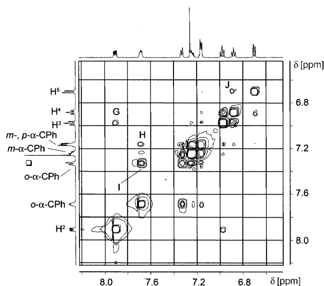
Figure 8. Expanded 2D ^1\text{H} - ^1\text{H} NOESY NMR spectrum of ( S )-7 ( \text{CDCl}_3 ). Selected aromatic-aromatic NOE interactions: G: \text{H}_2 - \text{H}_3 ; H: o - \alpha -Ph- m - \alpha -Ph; J: \text{H}_4 - \text{H}_5 . EXSY signal: I: o - \alpha -Ph- o - \alpha -Ph. Solvent signal: □, \text{CDCl}_3 .
